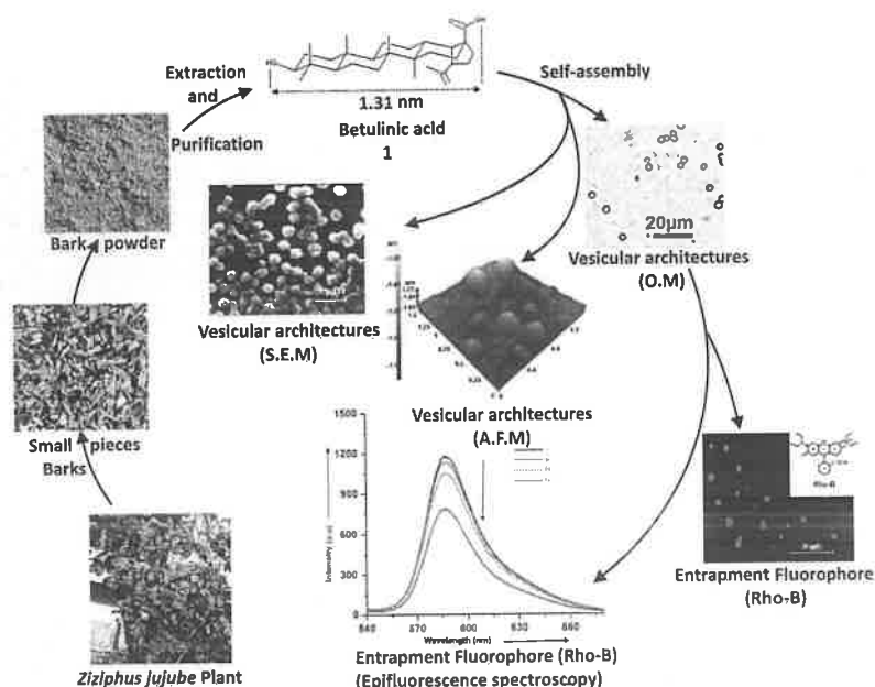
Figure 1: Schematic presentation of Self-assemblies of Betulinic acid 1, yielding vesicle like superstructures and application in removal of toxic dyes.
