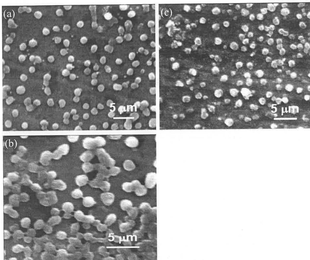
Figure 4. SEM images of dried self-assemblies of 1 in (a,b) DMSO-H 2 O (4:1v/v, 2 mM) and (c) DMSO-H 2 O (4:1v/v, 8 mM).
