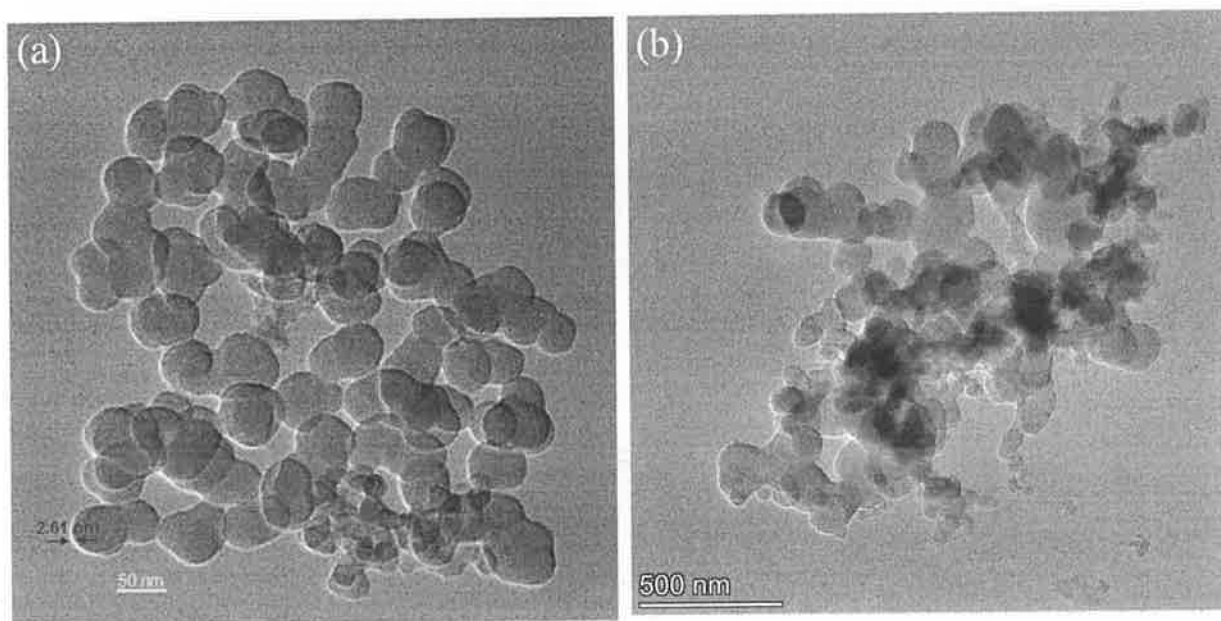
Fig. 5 HRTEM images of self-assembled 1 in DMSO- H 2 O (4:1 v/v, 1 mM, 0.045% w/v) at different magnifications (a,b). The membrane thickness measured was 2.61 nm, which is double of the molecular length of betulinic acid( 1.31 nm).
