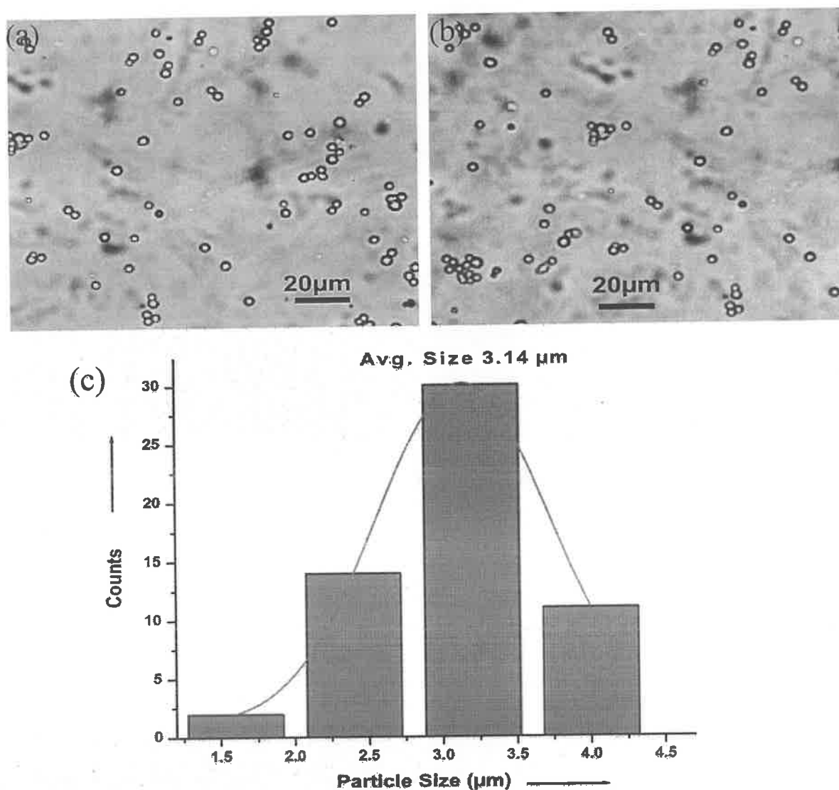
Figure 2. OPM images of self-assemblies of 1 : (a,b) in DMSO- \text{H}_2\text{O} (4:1, 43.09 mM) under normal light and (c) the plot of particle(vesicle like spherical objects) size vs counts in DMSO- \text{H}_2\text{O} (4:1), this inform us average diameter of spherical objects ( 3.14\text{ }\mu\text{m} ).
