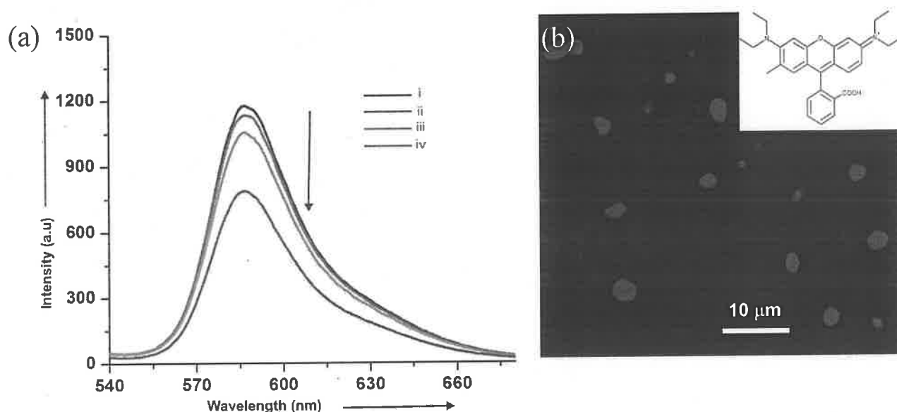
Figure 7: Entrapment of rhodamine-B by the vesicular self-assemblies of 1 in DMSO–H 2 O (2.29 mM, 4:1 v/v), (a) fluorescence emission spectra ( \lambda_{\text{max(ex.)}} 510 nm) at different time intervals: (i) free rhodamine-B (0.0229 mM), (ii) after 1 h, (iii) after 3 h and (iv) after 21 h. (b) Fluorescent images of vesicular self-assembled 1 (2.29 mM) containing rhodamine-B (0.0229 mM).
